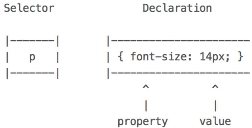
Figure 1: CSS Syntax
